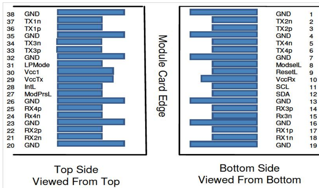
Figure 1. Pin function definitions
