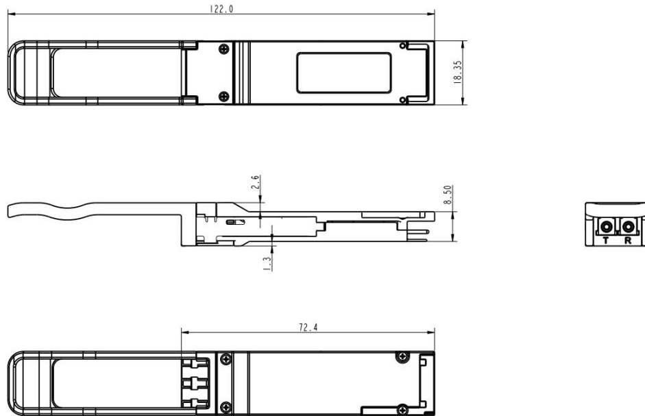
Figure 3. Module Mechanical Dimensions
