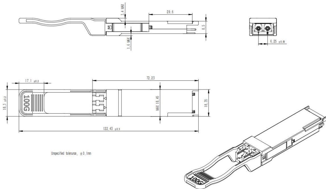
Figure 3. Module Mechanical Dimensions
