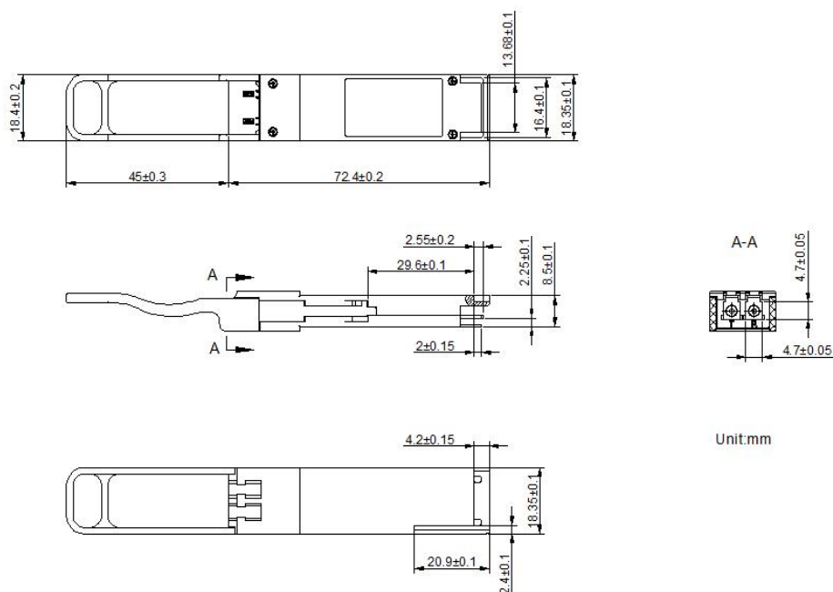
Figure 3. Module Mechanical Dimensions
