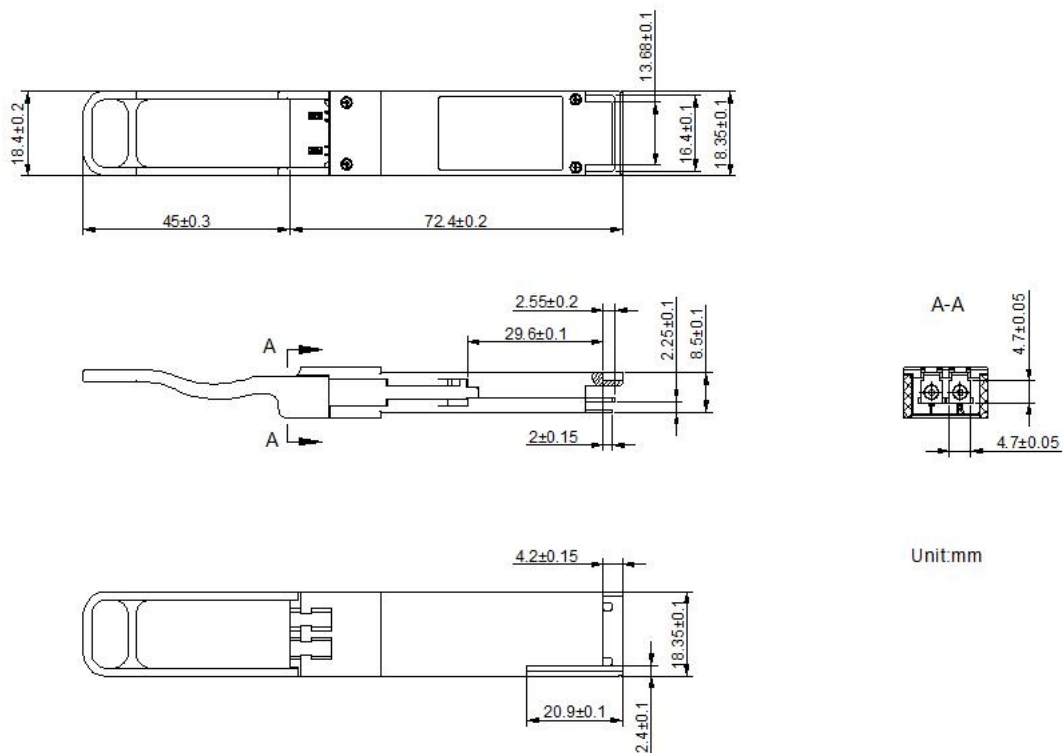
Figure 3. Module Mechanical Dimensions
