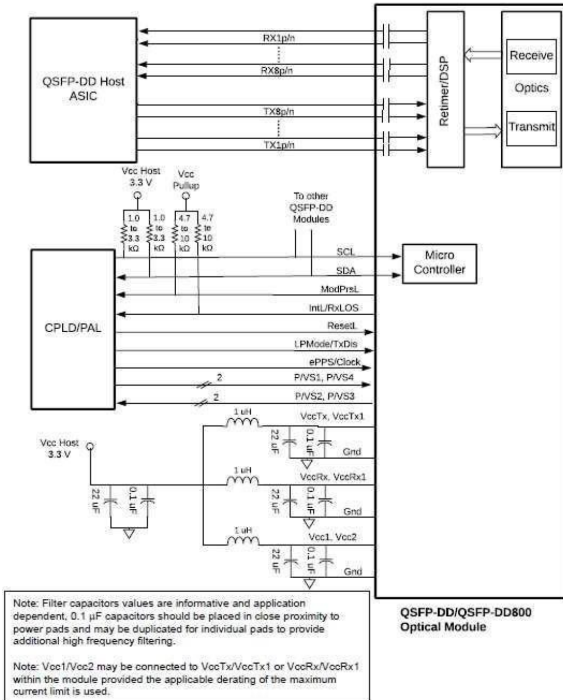
Figure 2 – Recommended QSFP-DD/QSFP-DD800 Host Board Schematic
