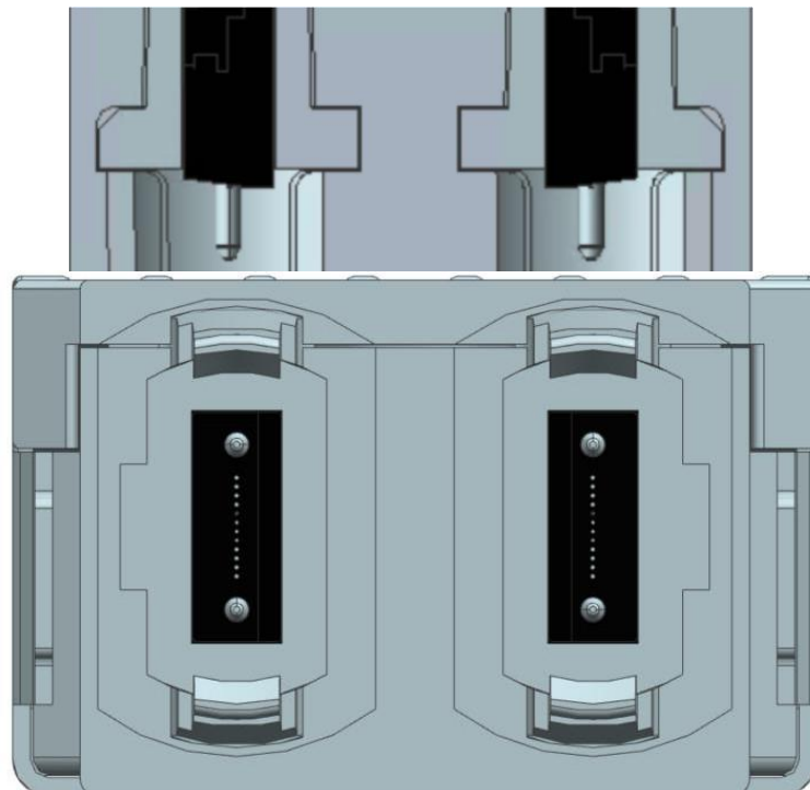
Figure 7.3.1 Dual MPO12 APC interface
