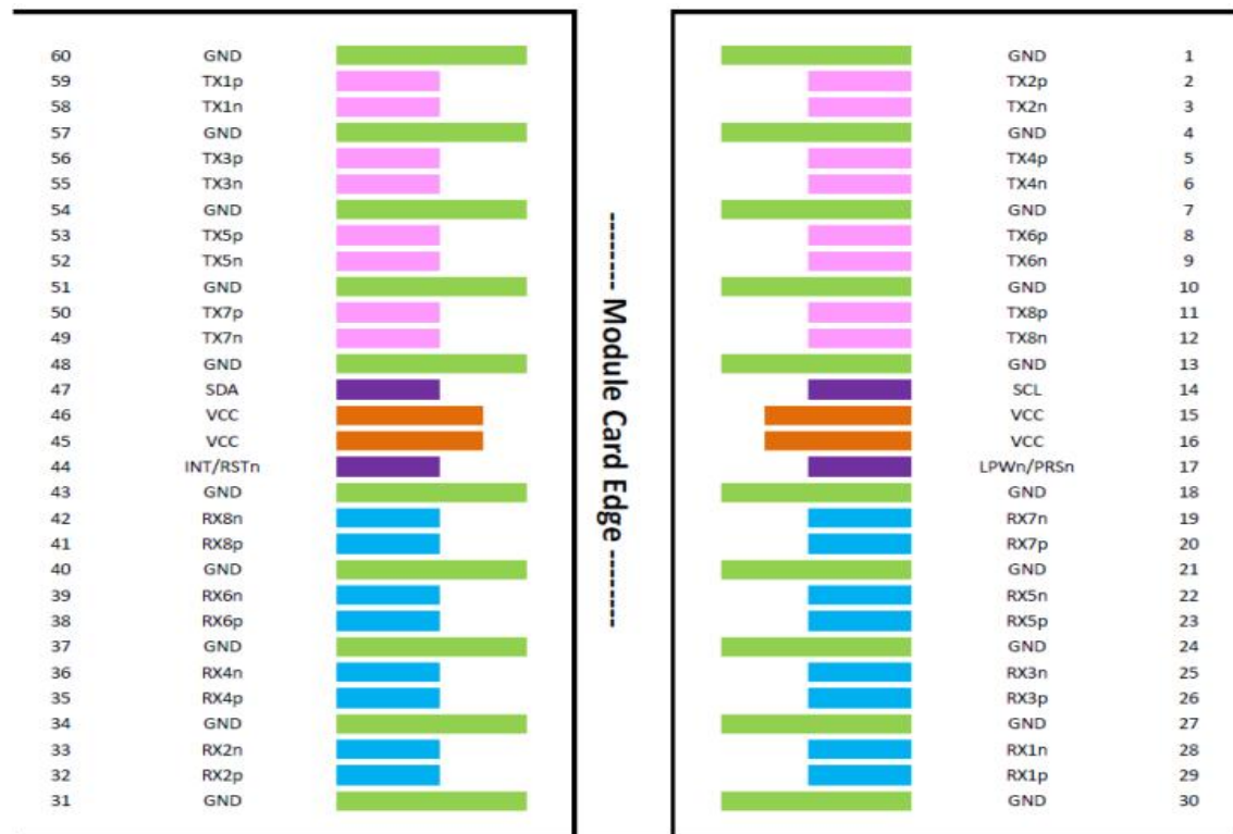
Figure 6.1 OSFP Transceiver Electrical Pad Layout
