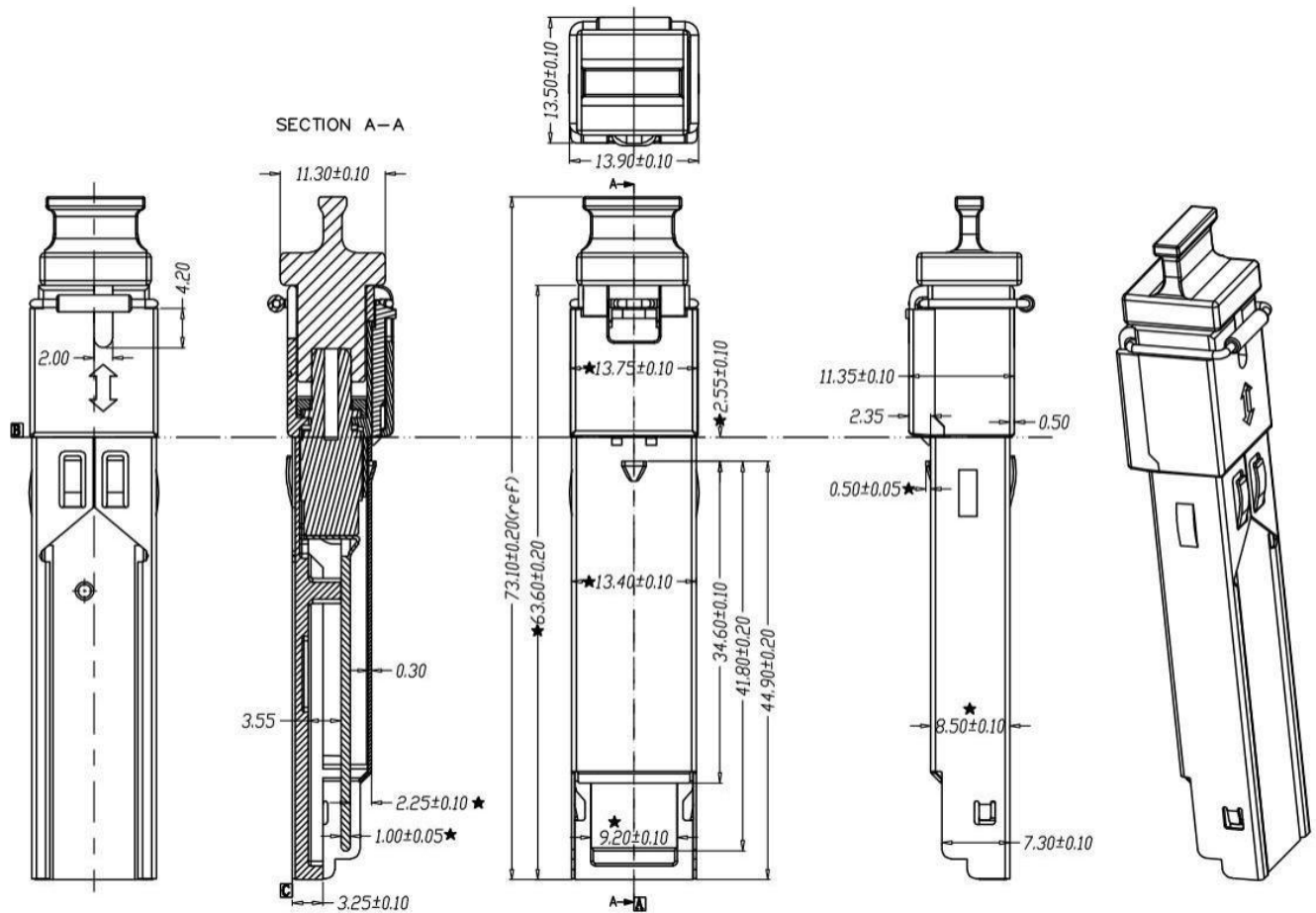
Figure 8, Mechanical Information
