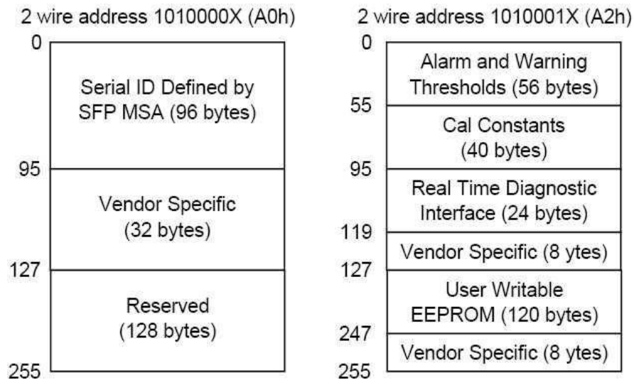
Figure 5, Memory map
