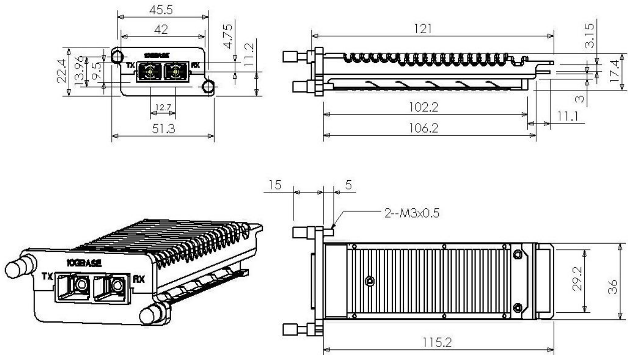
Figure 1 Mechanical dimensions
