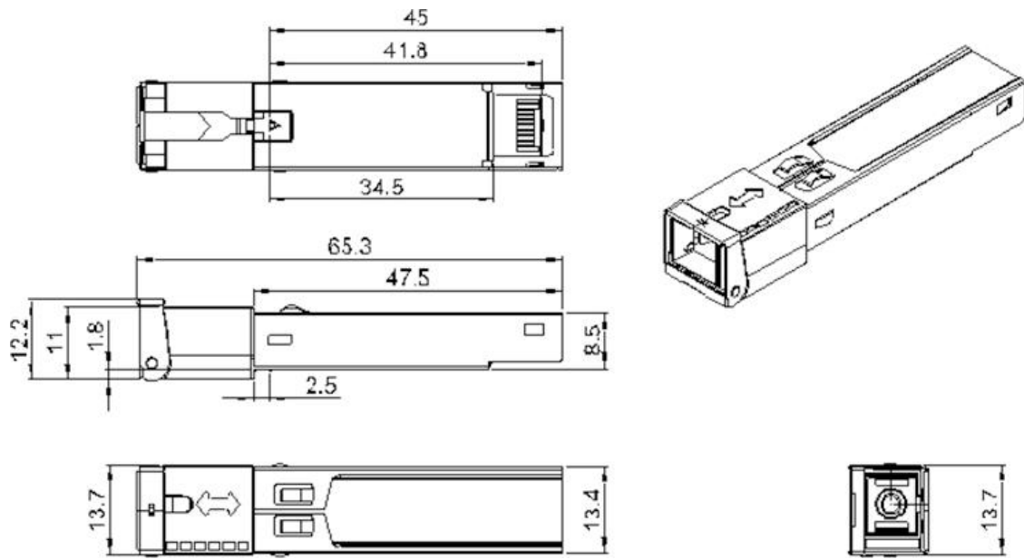
Figure 8 Package Outline
