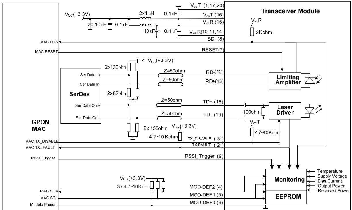
Figure 7 Typical Interface
