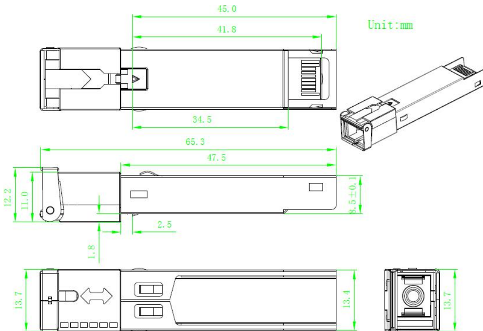
Figure 8 Package Outline
