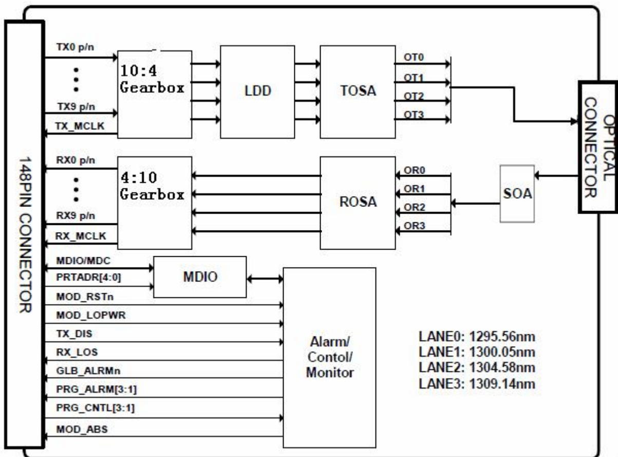
Figure 1. CFP ER4 Optical Transceiver functional block diagram
