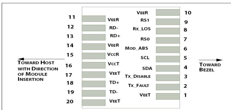
Figure 1. Host PCB SFP+ pad assignment top view
