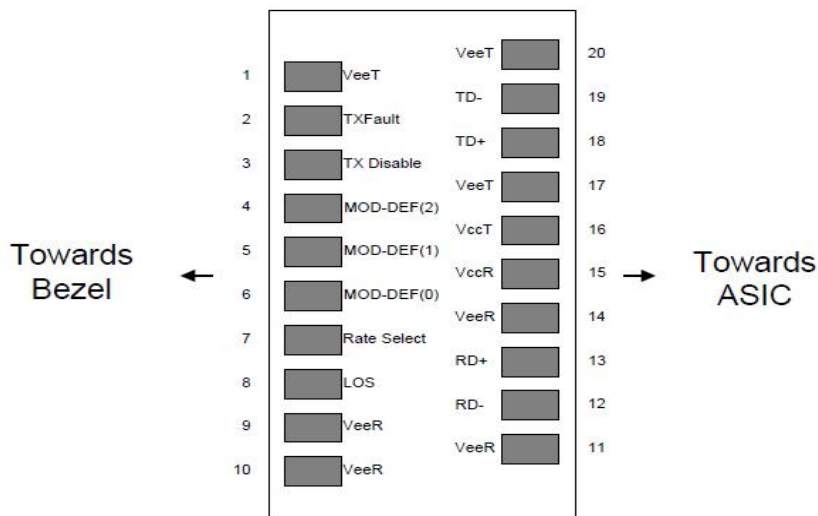
Figure 2: Pin-out of Connector Block on Host Board
